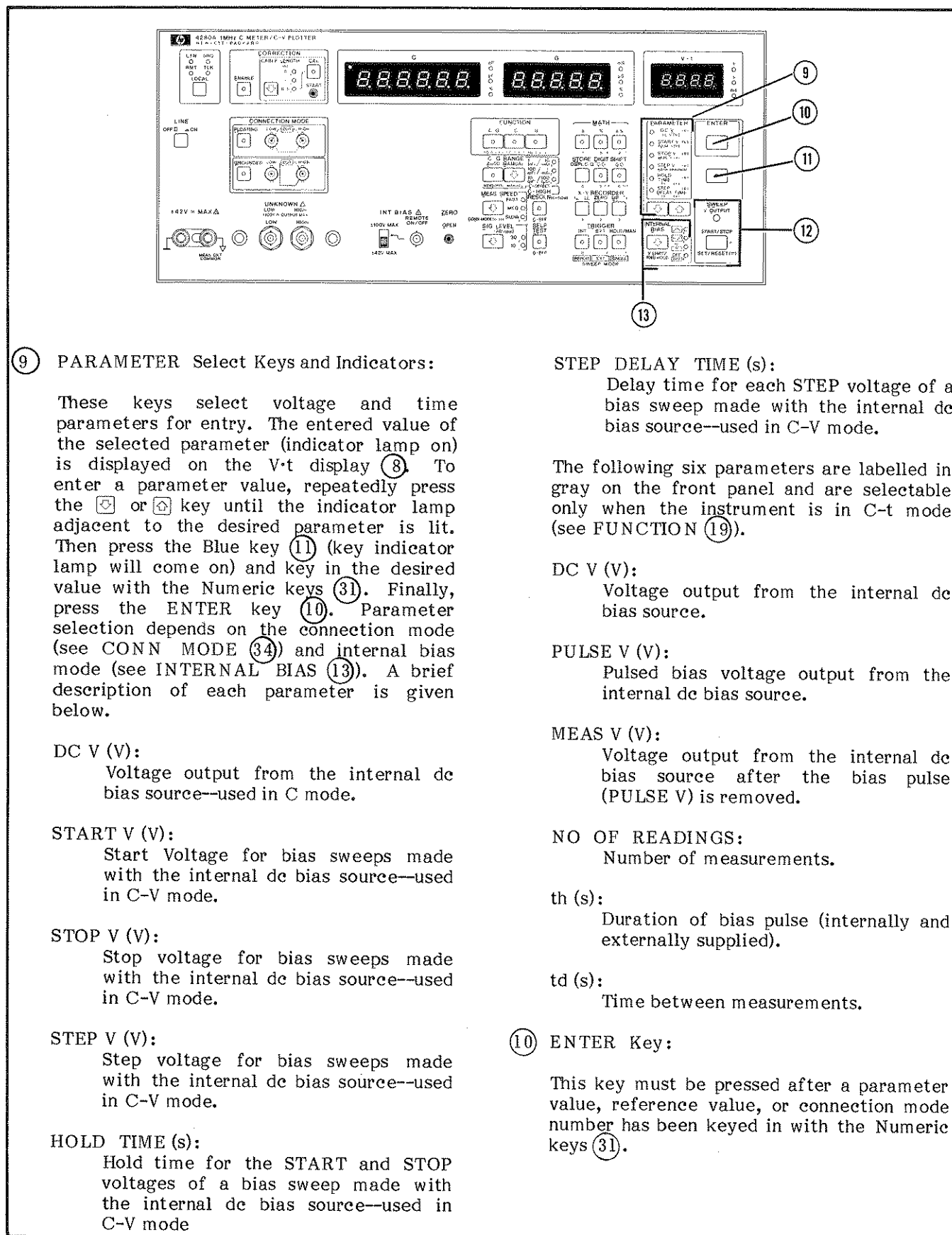
Figure 3-2. Front Panel Features (Sheet 3 of 12)
