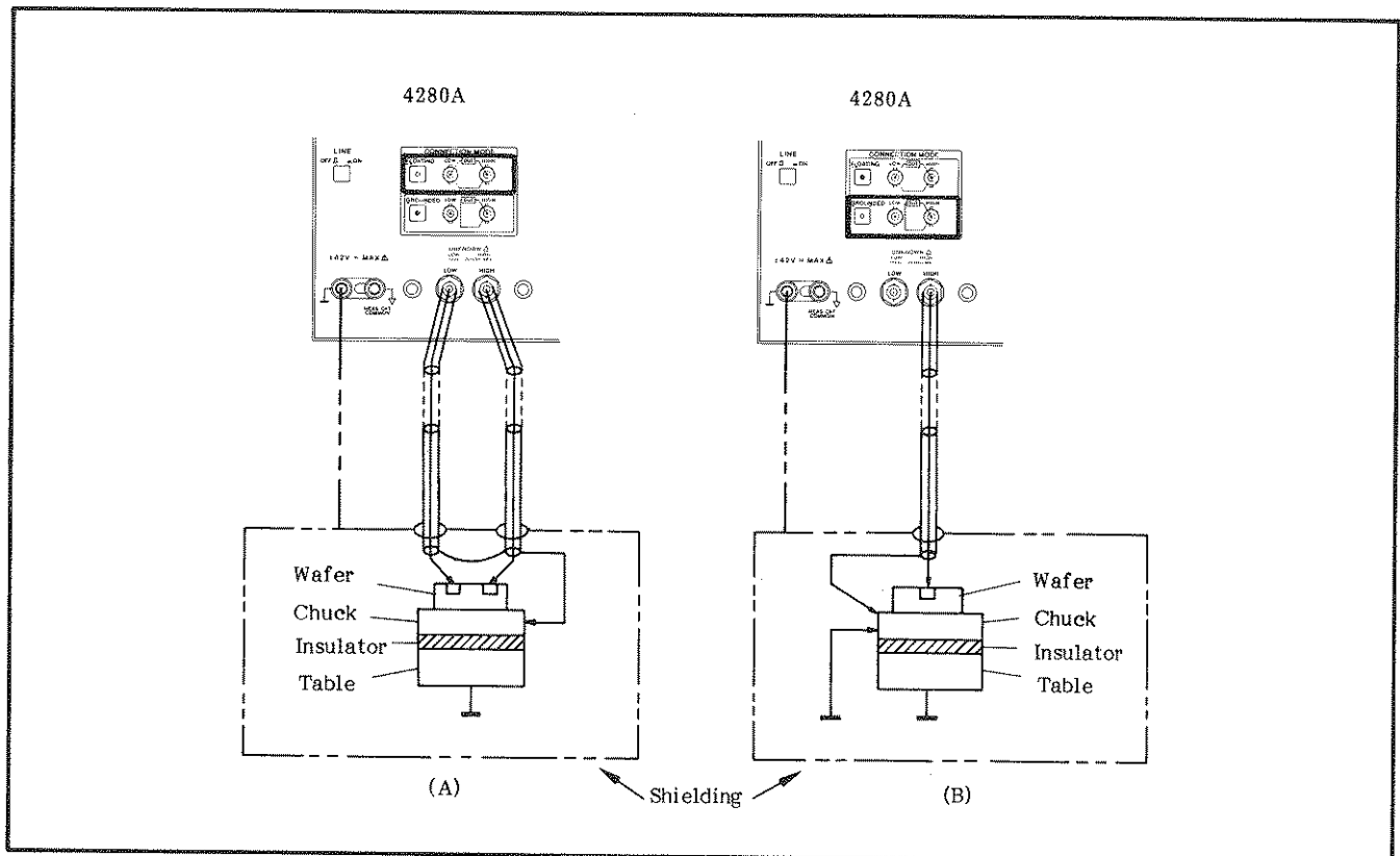
Figure 3-12. Connection Using a Wafer Prober
