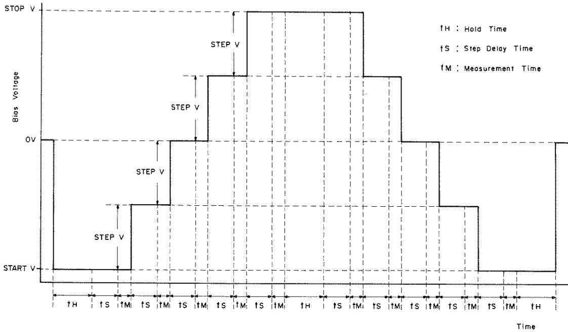
Figure 2. C-V Mode ( \square Bias Sweep)
