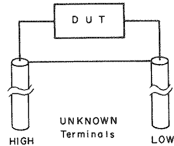
Figure 3-10. Floating Test Sample Connection
