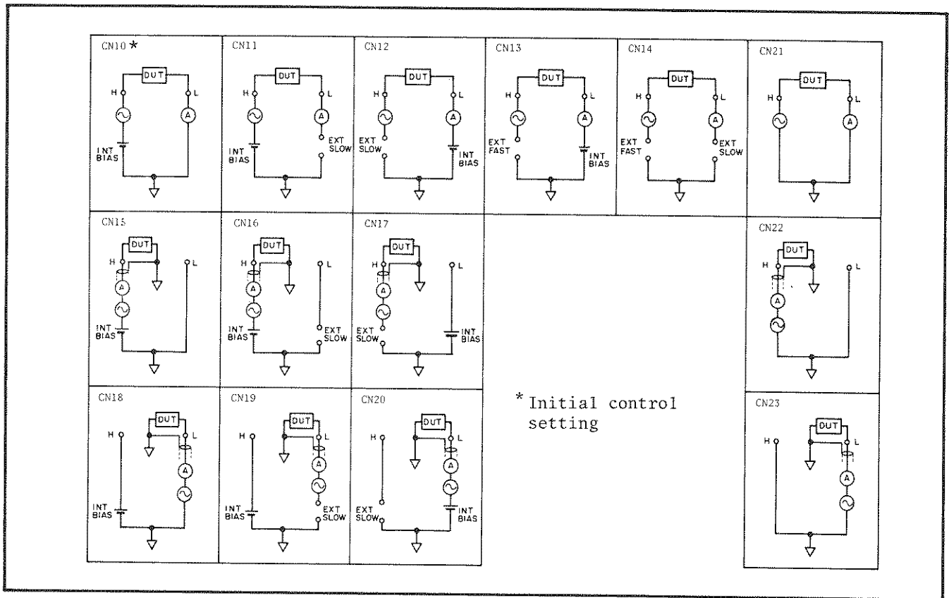
Figure 3-8. Connection Modes
