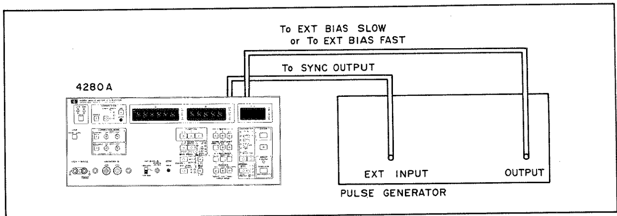
Figure 3-29. External Pulse Generator Connection
