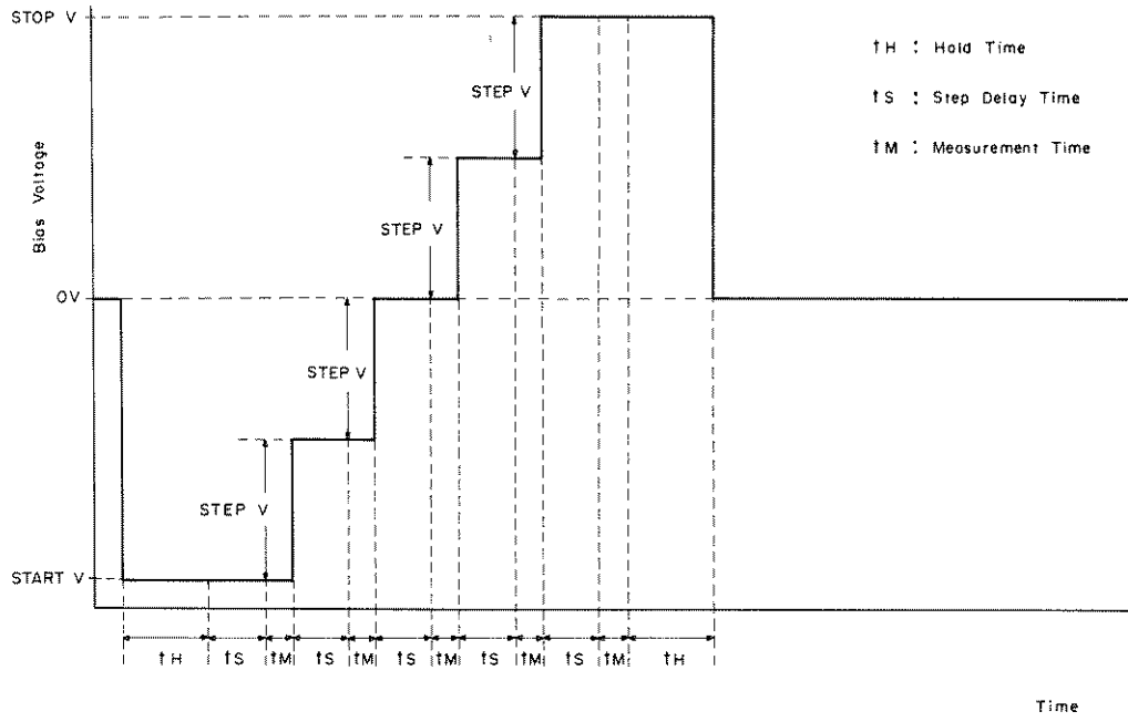
Figure 1. C-V Mode ( \square Bias Sweep)
