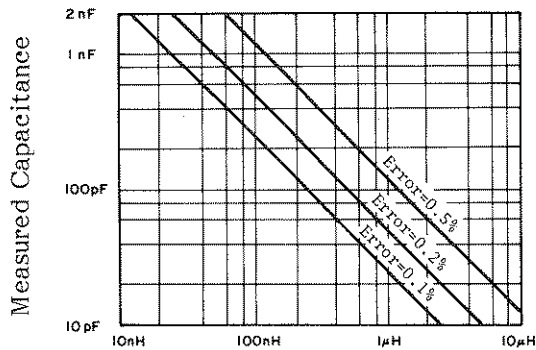
Residual Inductance
