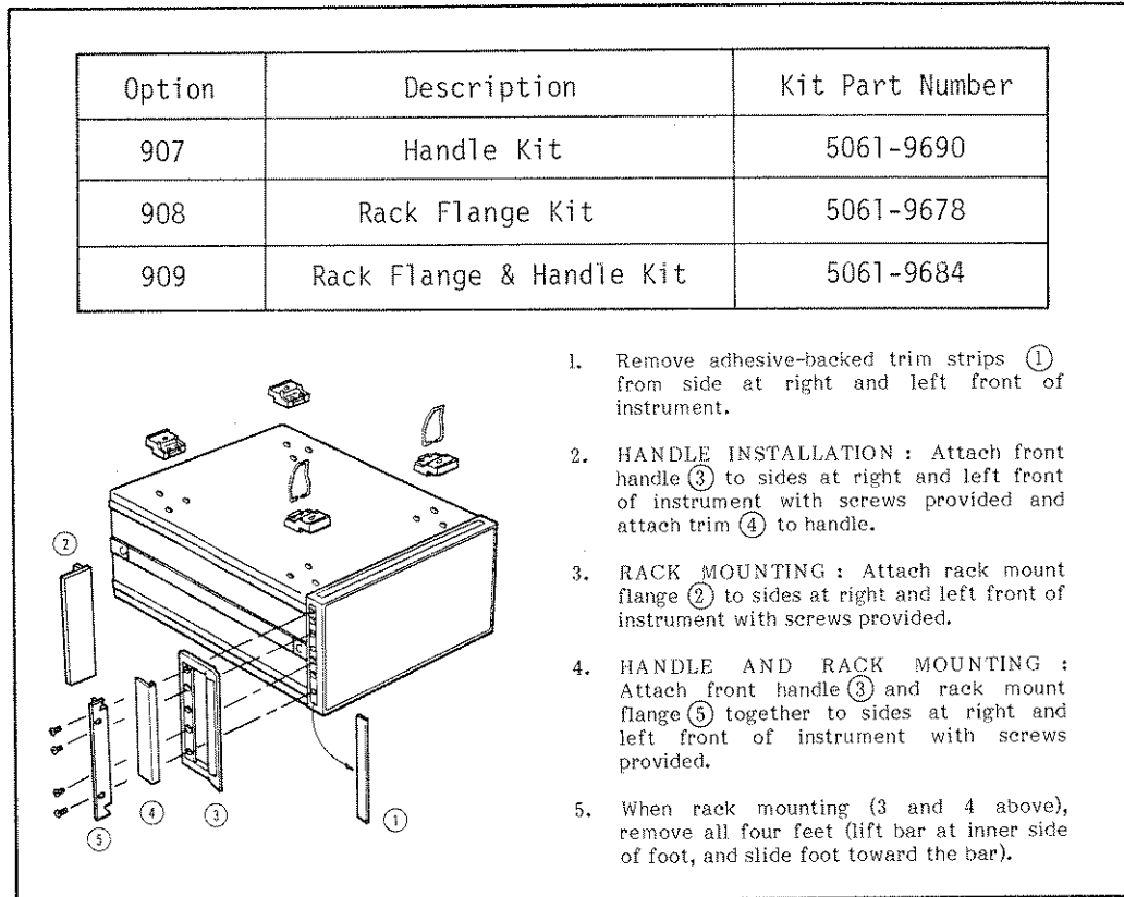
Figure 2-3. Rack Mount Kit
